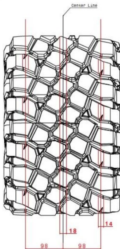
40. 40x12.50R17 | KR3 Mud01 Grooving Drawing
